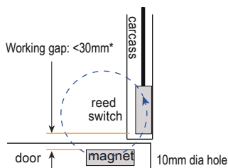
Fig 10: top view
