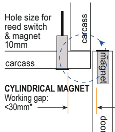
Fig 4: side view
