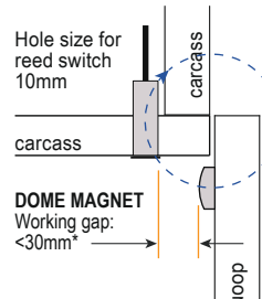
Fig 5: side view
