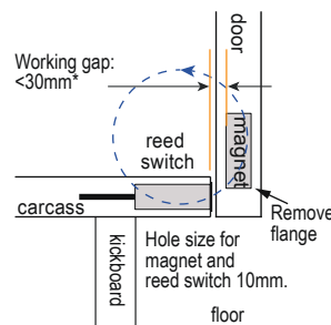
Fig 11: side view
